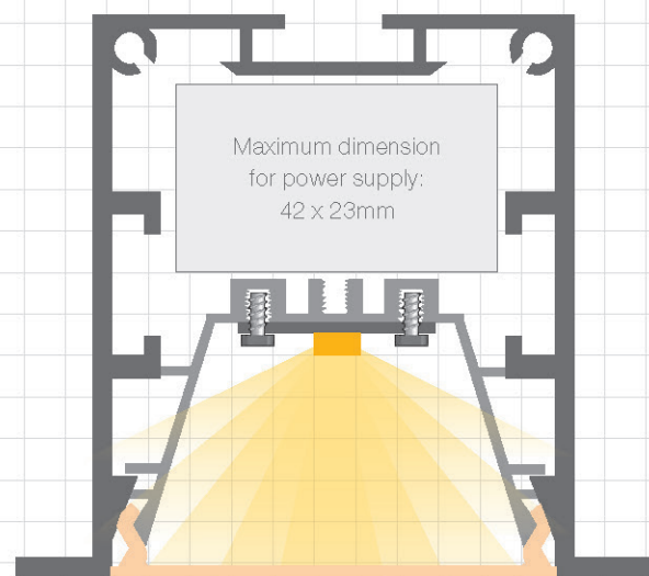
Krakovia 77 x 68 mm ○○●
