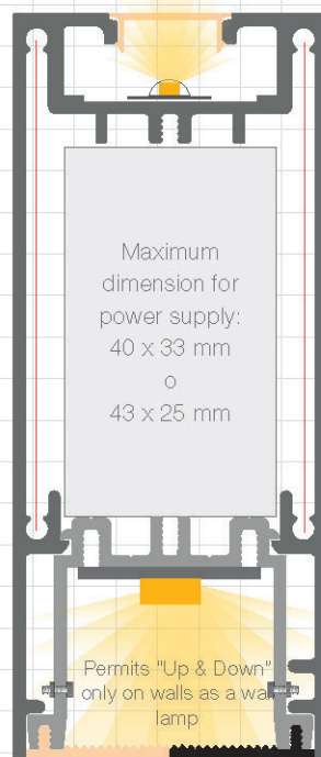
Munich Magnum Slim
