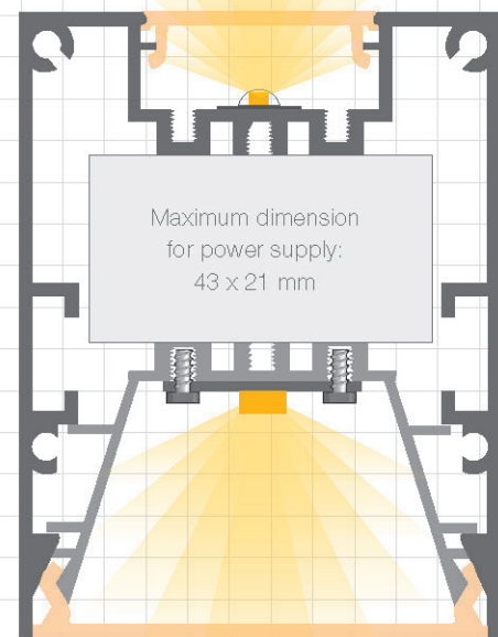
Liverpool 58 x 75 mm ○○●
