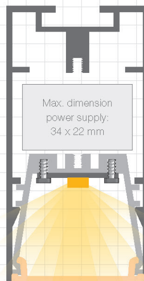
Gales Slim 39 x 75 mm ○○●
