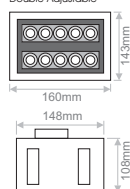
Lima 21W RC Double Adjustable
