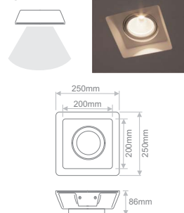
PCR.011 INVISIBLE SQUARE ADJUSTABLE
