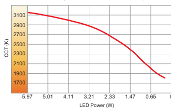
Warm dimming 3000K to 1800K (6W)
