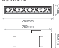
Lima 21W RC Single Adjustable
