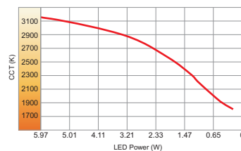
Warm dimming 3000K to 1800K (6W)
