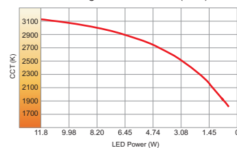
Warm dimming 3000K to 1800K (12W)
