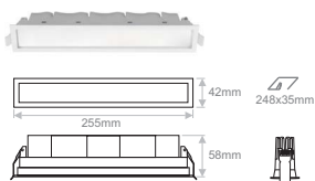
LIMA Diffused Recessed 21
