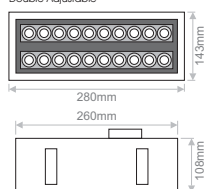
Lima 42W RC Double Adjustable
