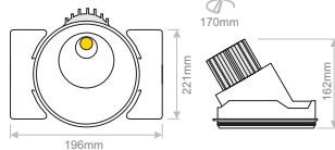
LUPO ROUND WASH 38W
