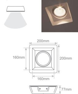
PCR.015 INVISIBLE SQUARE
