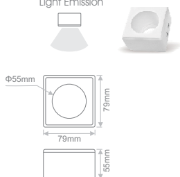
PCR.023 SHARP ROUND
