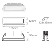
LIMA Diffused Recessed 10
