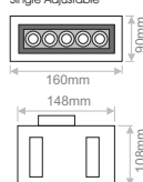
Lima 10W RC Single Adjustable
