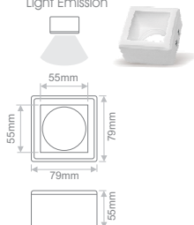
PCR.022 SHARP SQUARE
