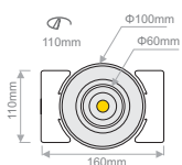
VERONA ROUND TRIMLESS
