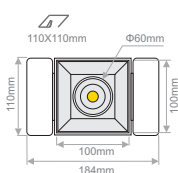
VERONA SQUARE TRIMLESS
