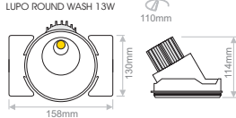
LUPO ROUND WASH 9W LUPO ROUND WASH 13W
