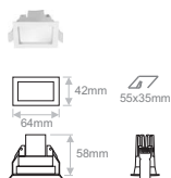
LIMA Diffused Recessed 4
