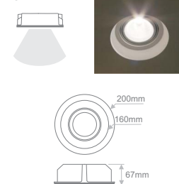
PCR.016 INVISIBLE ROUND
