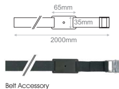
Belt Accessory
