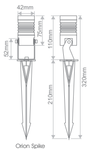
Orion Spike
