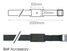
Belt Accessory
