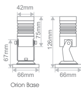
Orion Base
