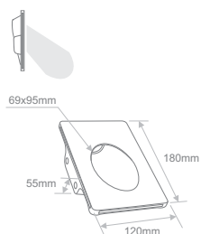
PWR.012 CERES L Light Emission
