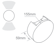
PWM.016 IDA Light Emission
