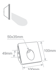
PWR.013 CERES Light Emission
