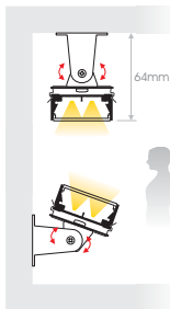
SURFACE installation
