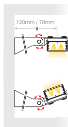
WALL BRACKET (Long/Short) installation
