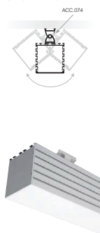
SURFACE WITH HINGE
