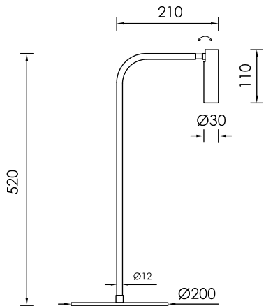
FERUS 20 BRASS
