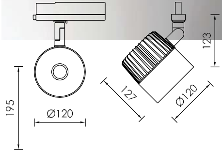
UBER 2 S.S.LED
